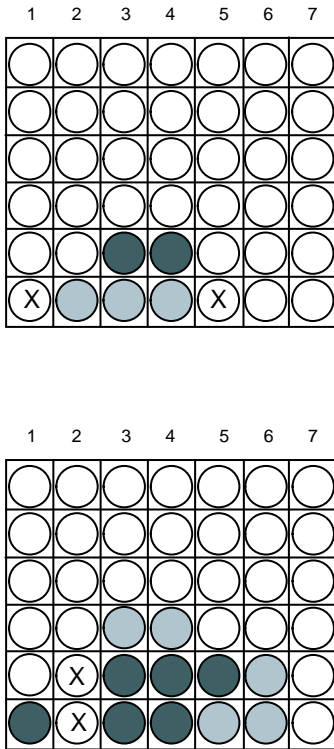
Fig. 1. Connect-Four Strategies
