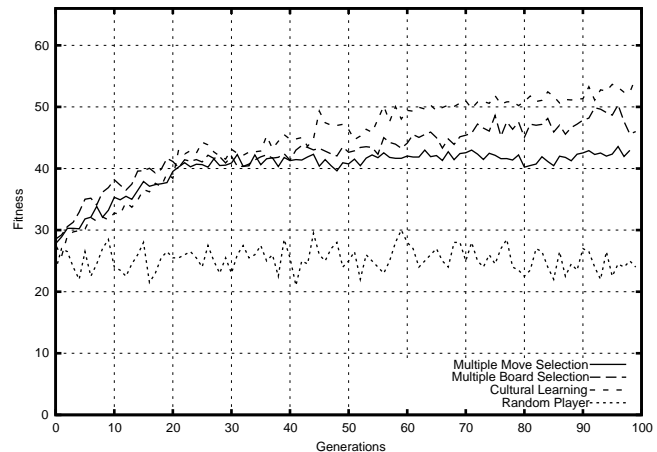
Fig. 6. Cultural Learning
