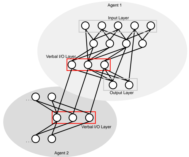
Fig. 3. Agent Communication Architecture
