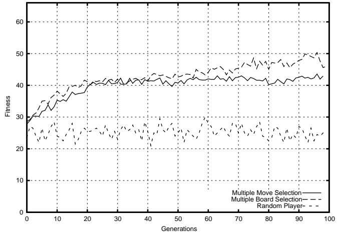
Fig. 5. Multiple Board Selection
